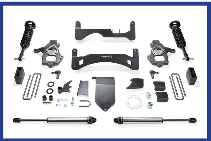
6" PERFORMANCE SYSTEM GEN II W/ DIRT LOGIC 2.5 COILOVERS
